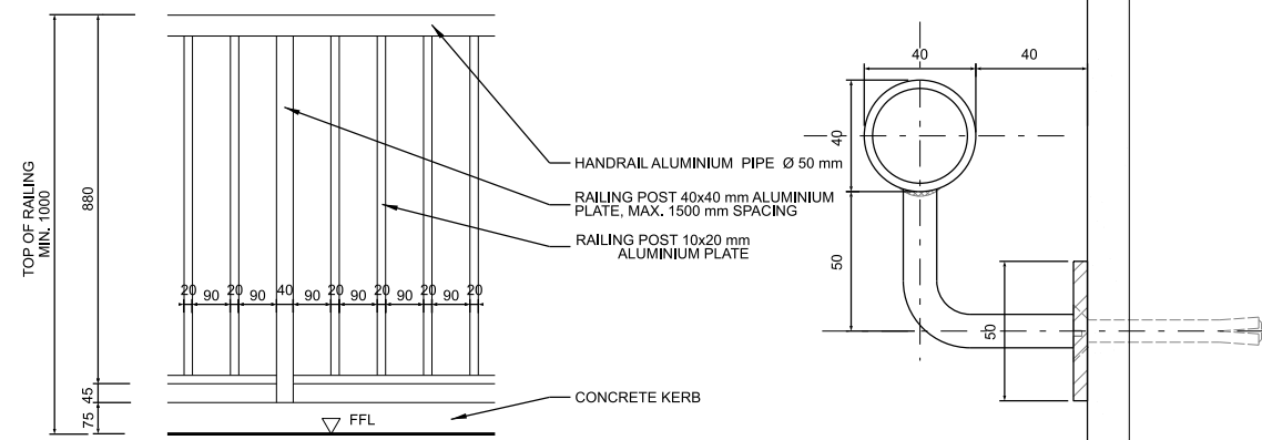
TYP. RAILING ON KERB DETAIL 1:10
