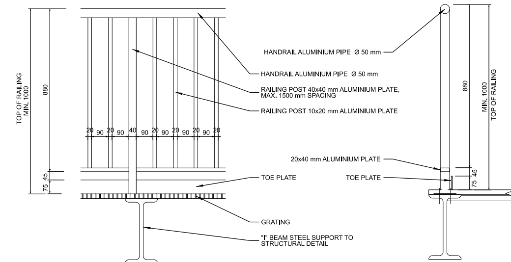
TYP. RAILING ON METAL PLATFORM DETAIL 1:10
