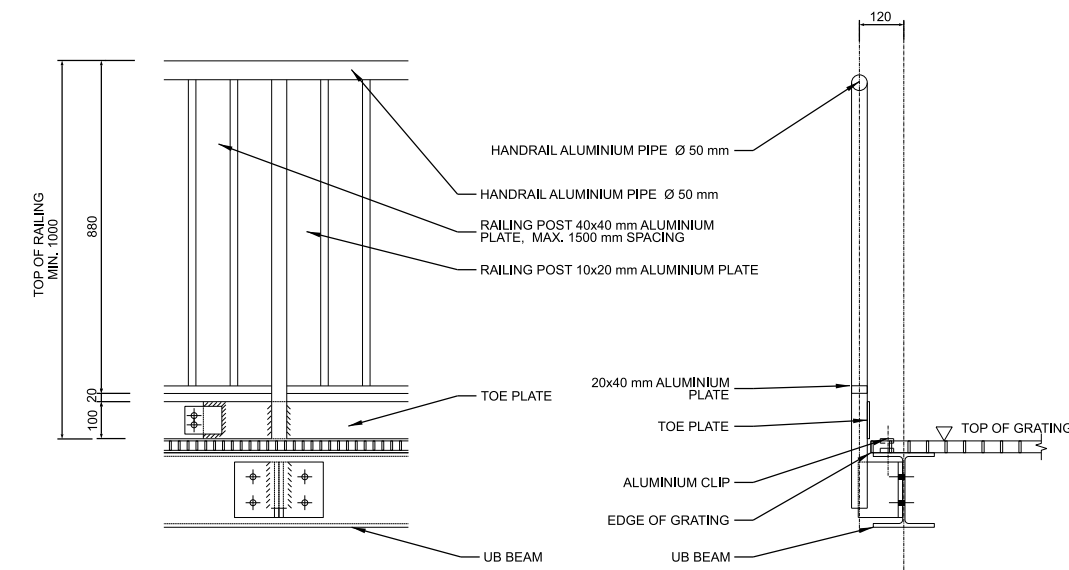
TYP. RAILING FOR CATWALK/PLATFORM 1:10
